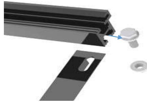
Image – 12: Aluminum profile connection
